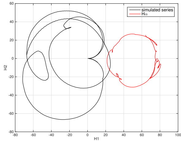
Figure 16. Simulation of two bidirectional coupled oscillators for the case of NGC 4151. Left: Random realization of Eq. (8) for two time series (black is U_a = OP1 , and red is U_b = OP2 ) of amplitudes A = 6.09 , B = 1.04 , phase \phi = 2.2 \text{ rad} , coupling strengths cp_{a \rightarrow b} = 0.7 , cp_{b \rightarrow a} = 0.6 , periods are 500, 300 and time delay is 100 arbitrarily chosen time units. Note the similarity of sharpness of this signal 'bursts' with features in the observed light curves. Right: corresponding 2D correlation map .
