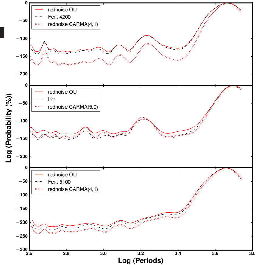
Fig. 2 Bayesian periodograms of the simulated 'red noise' and real light curves on a logscale.
