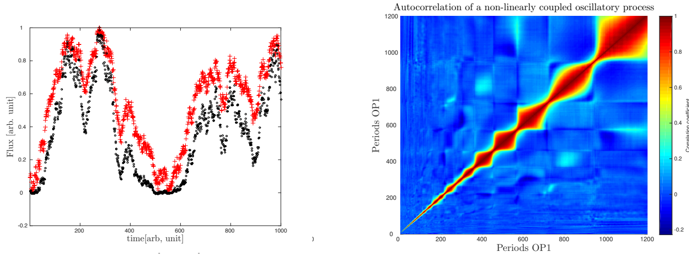
Figure 16. Simulation of two bidirectional coupled oscillators for the case of NGC 4151. Left: Random realization of Eq. (8) for two time series (black is U_a = OP1 , and red is U_b = OP2 ) of amplitudes A = 6.09 , B = 1.04 , phase \phi = 2.2 \text{ rad} , coupling strengths cp_{a \rightarrow b} = 0.7 , cp_{b \rightarrow a} = 0.6 , periods are 500, 300 and time delay is 100 arbitrarily chosen time units. Note the similarity of sharpness of this signal 'bursts' with features in the observed light curves. Right: corresponding 2D correlation map .
